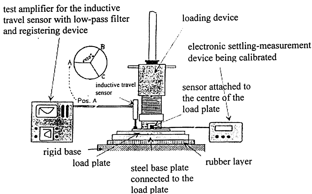
Figure 4. Simplified drawing showing the set-up for the calibration of the settling-measurement device
